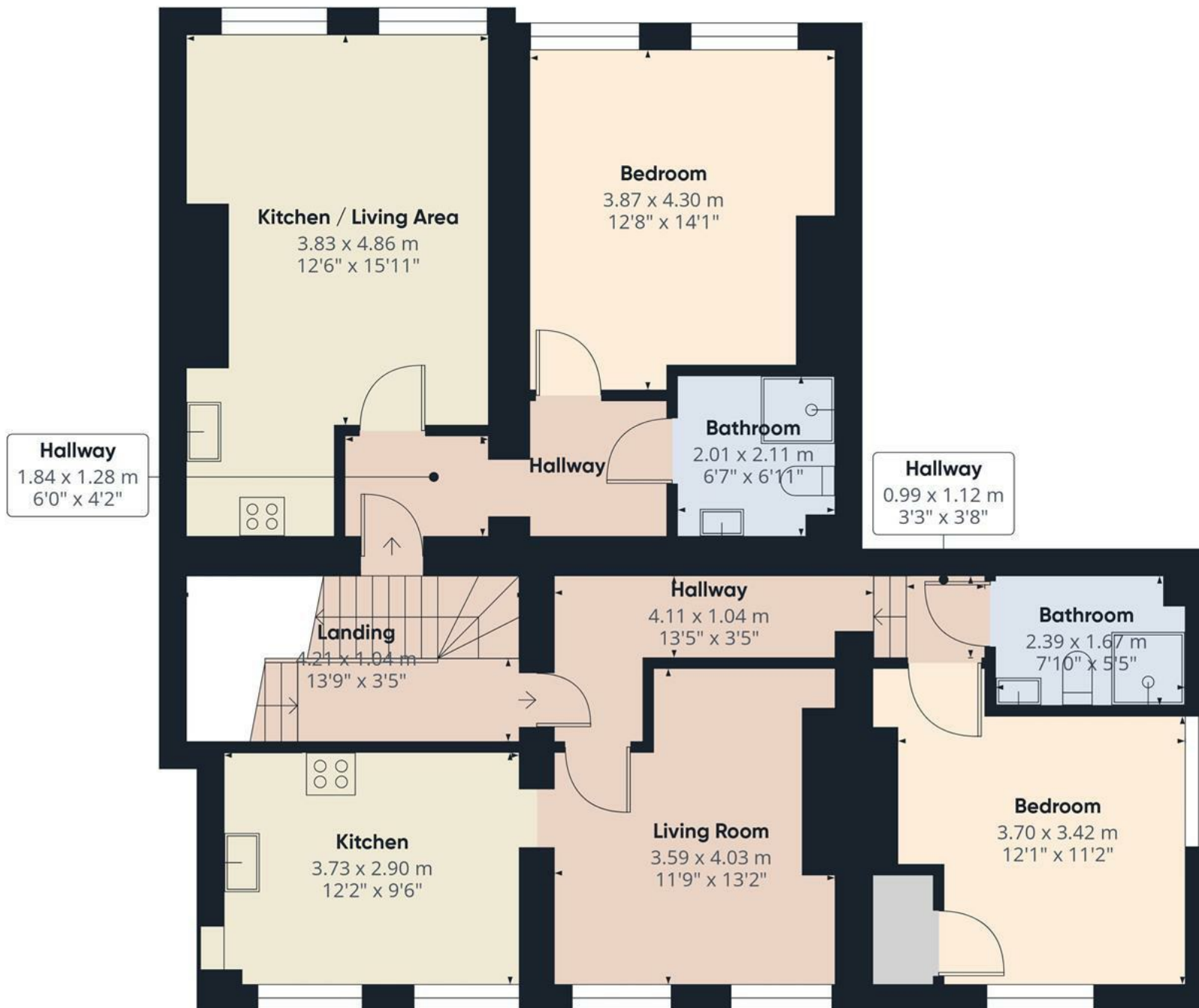
Floor 2
